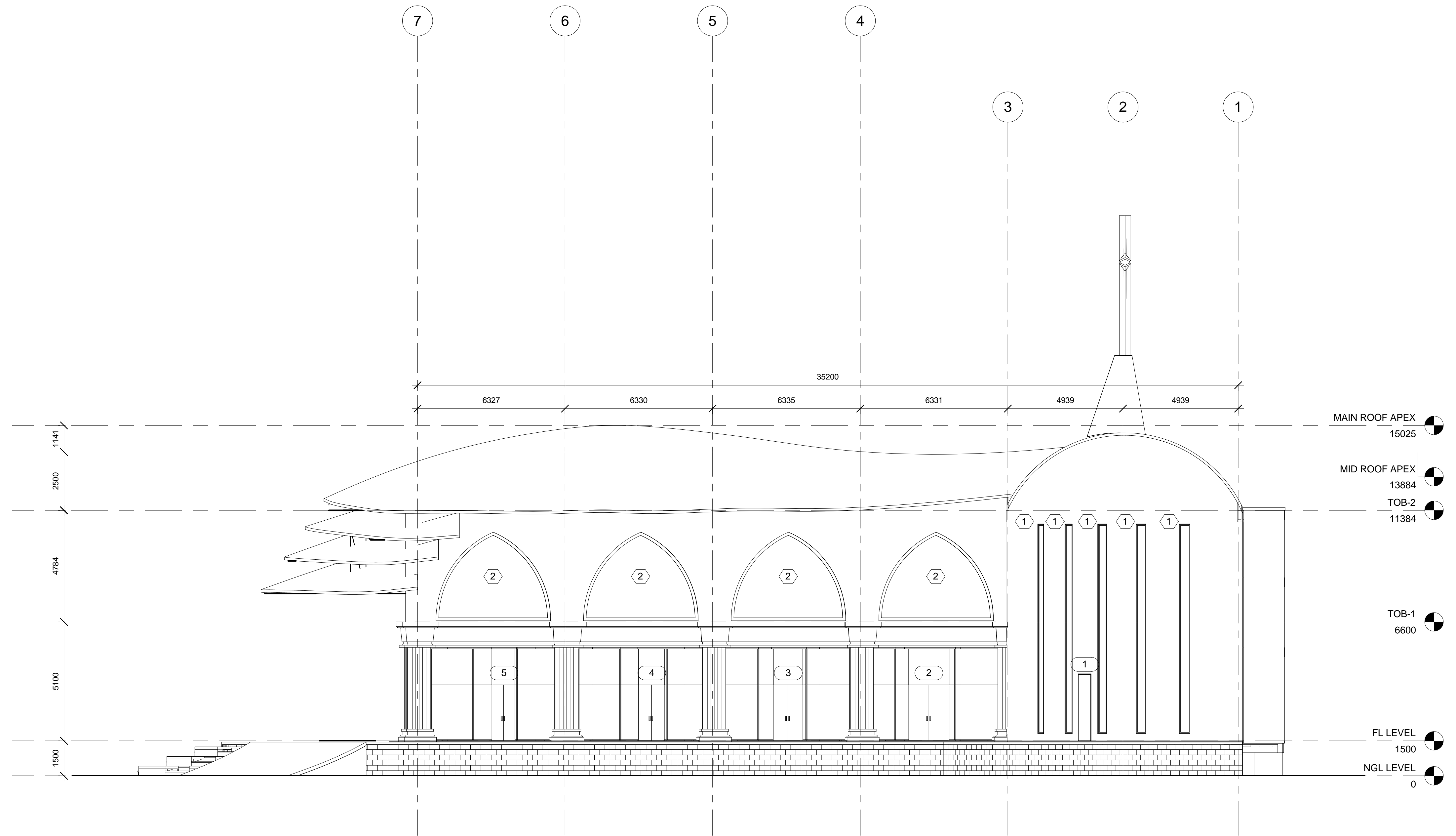
2 RIGHT SIDE ELEVATION 1 : 100
