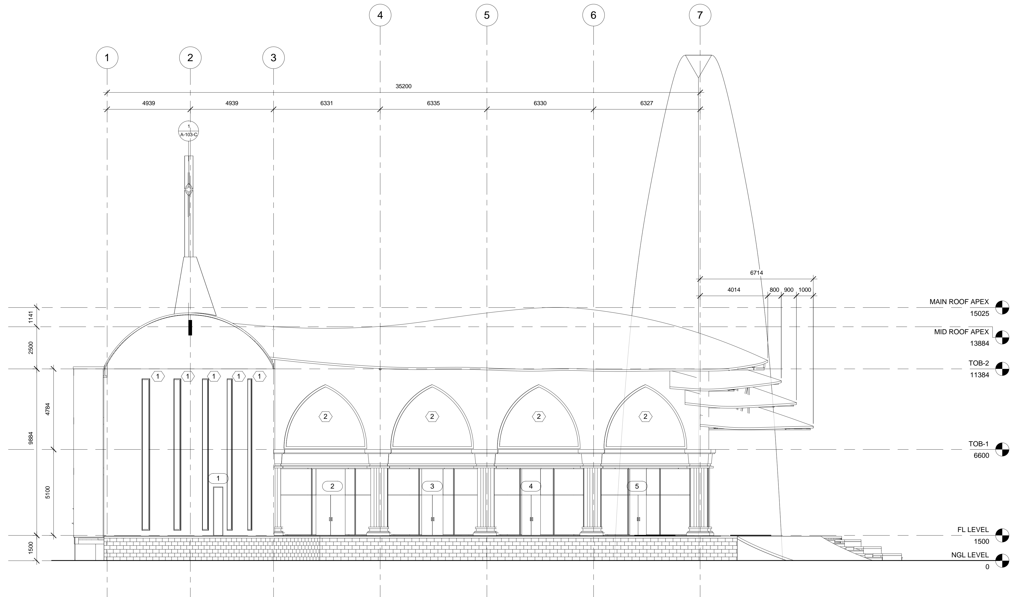
1 LEFT SIDE ELEVATION 1 : 100
