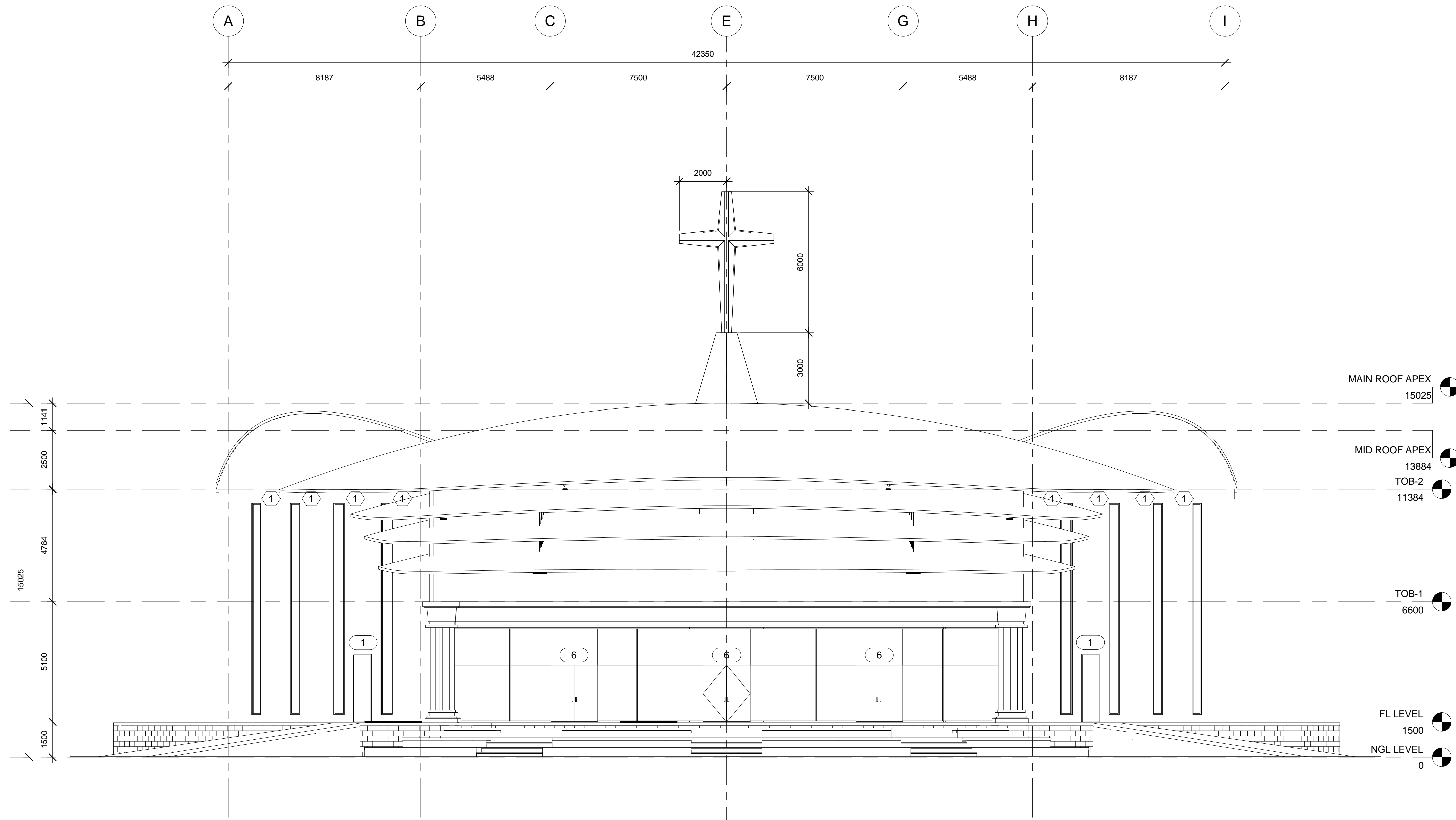
1 FRONT ELEVATION 1 : 100
